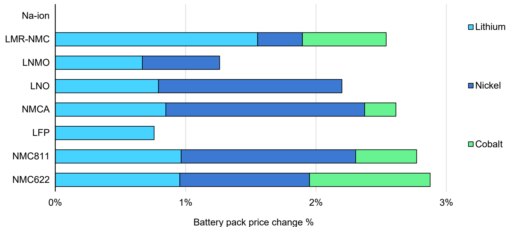
Impact of 10% commodity price change on the battery pack price for selected battery chemistries
